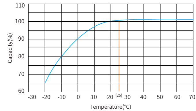
Temperature Effects on Capacity at 75A
