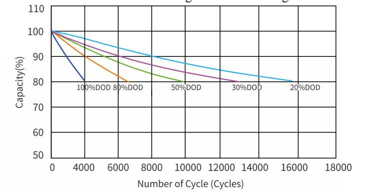
Cycle Life with DOD at 25°C 150A Discharge and 150A Charge
